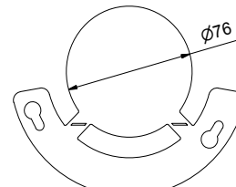
Restrictor B Ø76
