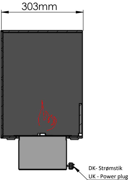
SECTION BB-BB SCALE 1 : 8
