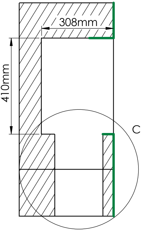
SECTION B-B
