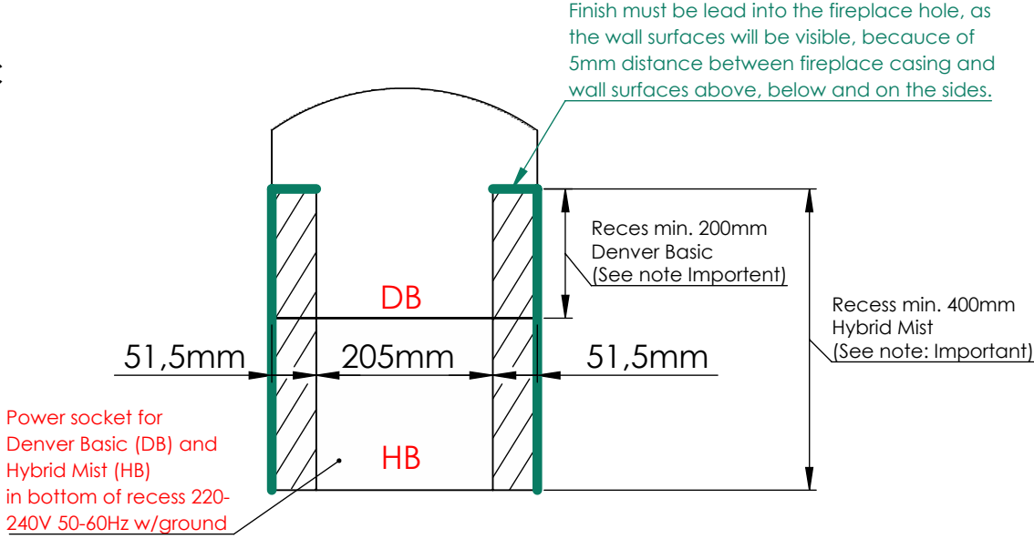
UK recess - DETAIL C SCALE 1 : 8
