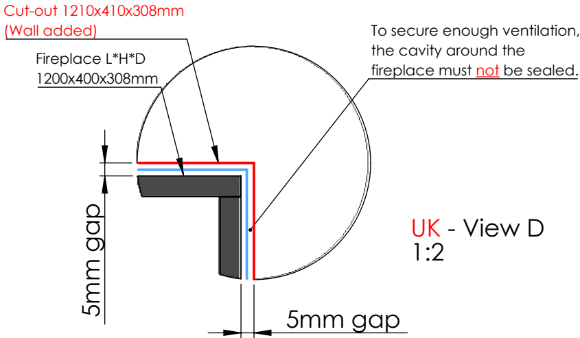
UK - Fireplace incl. wall
