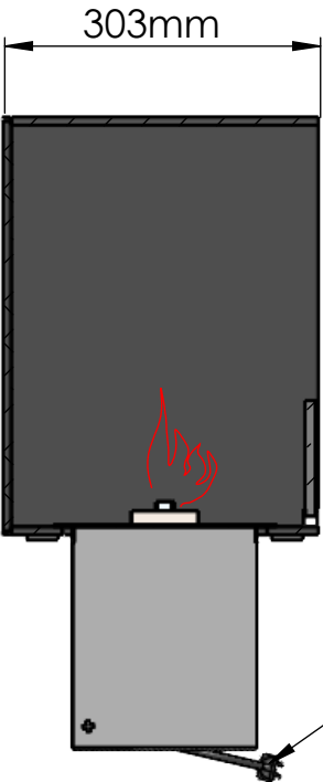
SECTION BB-BB SCALE 1 : 8
