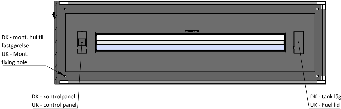
SECTION AA-AA SCALE 1 : 8
