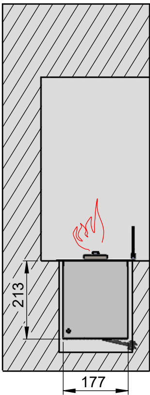
SECTION AI-AI
